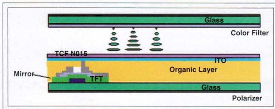
Fig. 6: Sony demonstrated this transfective TFT-LCD employing one internal TCF TM polarizer and two external conventional sheet polarizers at SID 2004.
