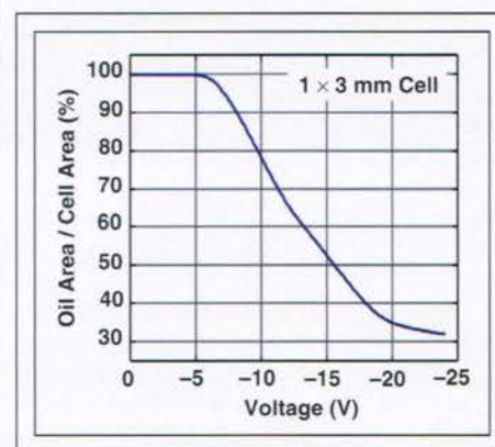
Fig. 3: A typical ELV voltage response is shown. Smaller-sized ELVs can modulate the oil area to as little as 10%. Less than 10-V ELV operation has also been demonstrated.
