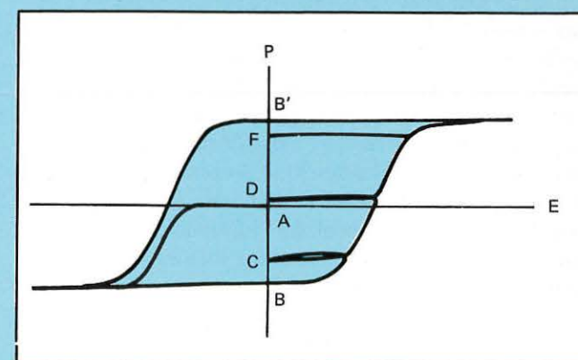
Fig 2 In the polarization (P) vs electric field (E) hysteresis loop, the net polarization is zero in the virgin or thermally depoled state (A). Applying a negative electric field increases the polarization (negatively) until it saturates at the maximum applied field. Removing the field, poles the ceramic to negative saturation remanence (B). Remanent polarization can be switched incrementally through intermediate values, e.g., (C), (D) and (F), to positive saturation remanence at (B') by application of a positive electric field.
