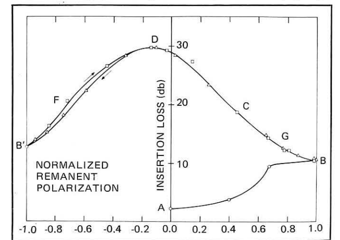
Fig 5 Insertion loss in dB plotted as a function of the normalized remanent polarization P_r/P_R for a PLZT 7/65/35 ceramic plate. Note that insertion loss in dB can be divided by 10 to obtain optical density.
