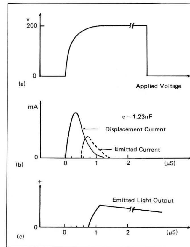
Fig 5 Wave form of applied voltage, displacement current, emitted current and emitted light output observed with EL device.
