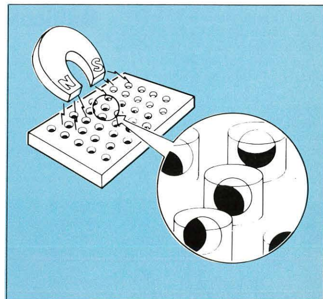
Fig 1 Principle of the magnetic particle display. Each spherical particle dark-colored in one hemisphere and light in the other is a tiny permanent magnet, free to rotate.
