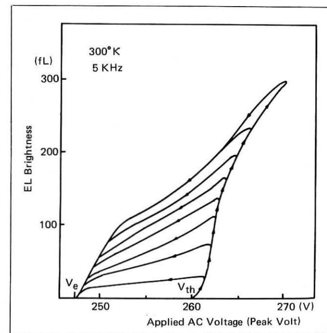
Fig 6 Hysteresis behavior observed in the EL brightness vs. voltage amplitude characteristics under square wave excitation.
