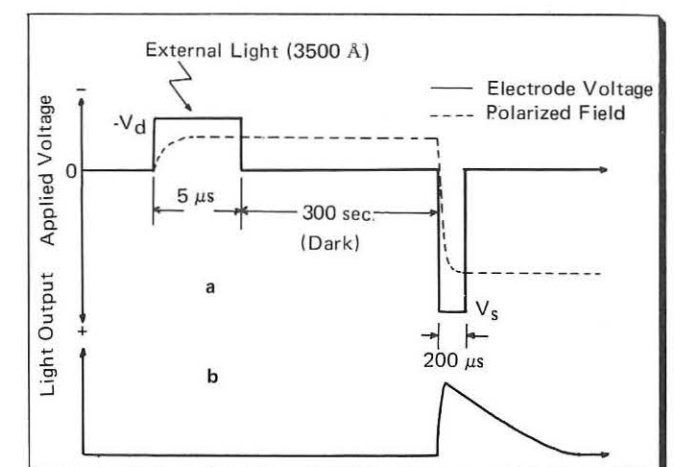
bias of Vd as parameter, is illustrated in Fig 12. The readout pulse has a constant pulse width of 200 microseconds, and the output light is in arbitrary scales.
