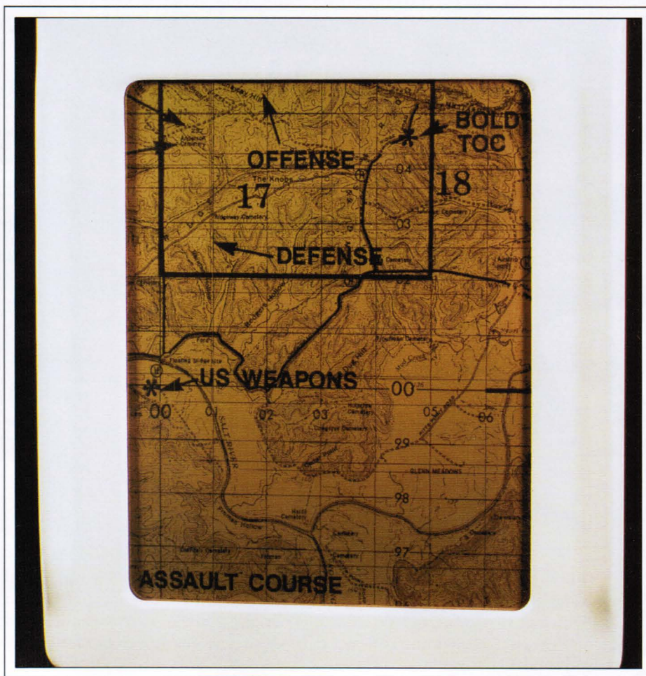
Fig. 1: Kent Display Systems, Kent State University, and the University of Stuttgart jointly developed this reflective 8½ × 11-in., 100-dpi, monochrome Ch-LCD. The display requires no backlight and is bistable – it requires power only to write a new image, not to retain it or view it – so its power consumption is 1/50 that of a comparable TN or STN display.
