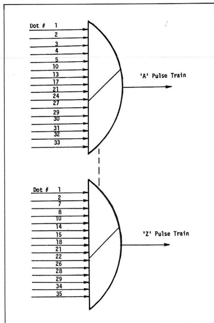
Figure 6: Character encoder.
