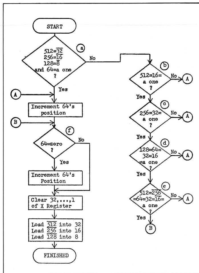
Figure 14: Tabulate algorithm.
