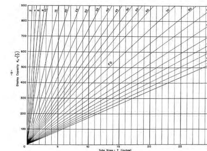
FIGURE 5: Display capacity as a function of CRT tube sizes and viewing conditions (3:4 aspect ratio).
