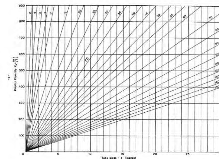
FIGURE 4: Display capacity as a function of CRT tube sizes and viewing conditions (4:3 aspect ratio).
