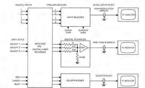
FIGURE 3: Basic system using only 8 tracks.
