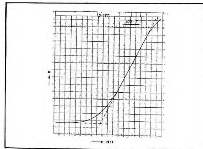
FIGURE 1: Density D vs. exposure Ht for an Eastman Kodak Spectroscopic plate type 103-F developed = 1.97, Maximum density above gross fog = 2.9; log scale for Ht .
