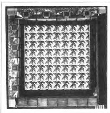
Fig. 2: The plasma panel and address drive circuits used in the briefcase computer. Only 8 Supertex HV03 high-voltage IC drivers (each of which consists of 64 n-channel open-drain high-voltage transistors and the associated shift register), are needed to address this 512x512 panel.
