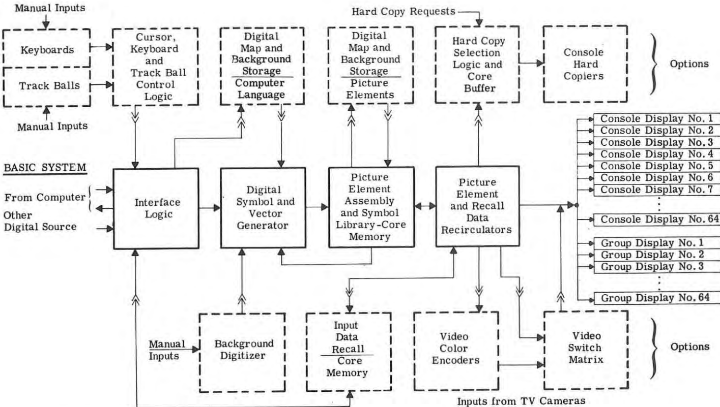
FIGURE 3: Precision digital television display systems.
