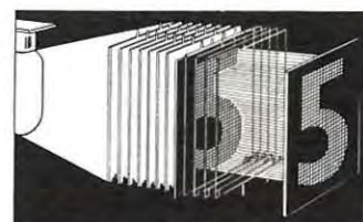
The Bina-View employs a light interference technique as illustrated.
