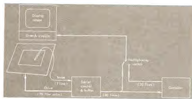
FIGURE 10: Information Paths in Graphic I/O System
