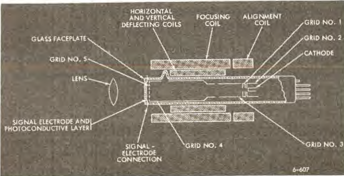
FIGURE 1: Vidicon tube.
