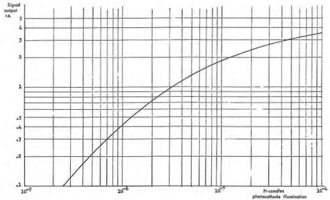
FIGURE 6: Transfer characteristic, image intensifier orthicon RCA C74003.
