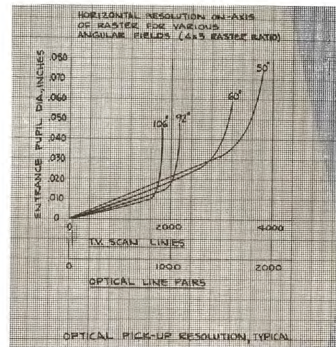
FIGURE 5: Optical pick-up resolution, typical.
