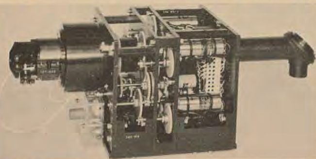
FIGURE 6: Optical pick-up.
