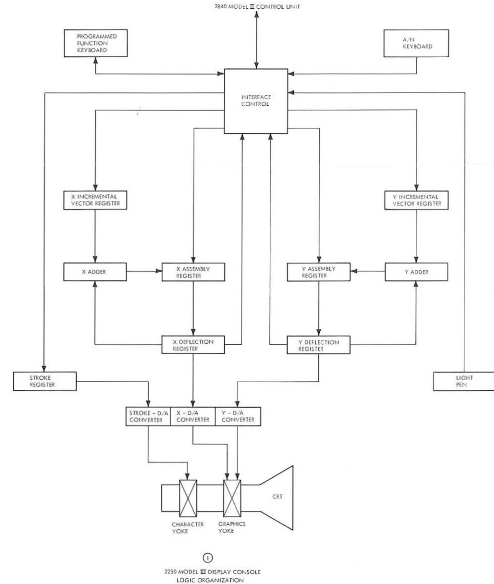
FIGURE 9: The 2250 III display console contains the logic, magnetic deflection system, manual-input devices and power supplies. Adders are used to compute the next character position and to convert incremental-mode vectors into absolute X-Y screen coordinates. Accumulation of the next vector in the assembly registers is overlapped with beam deflection for the previous vector.
