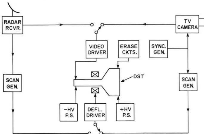
FIGURE 9: DST approach to multi-sensor display system.
