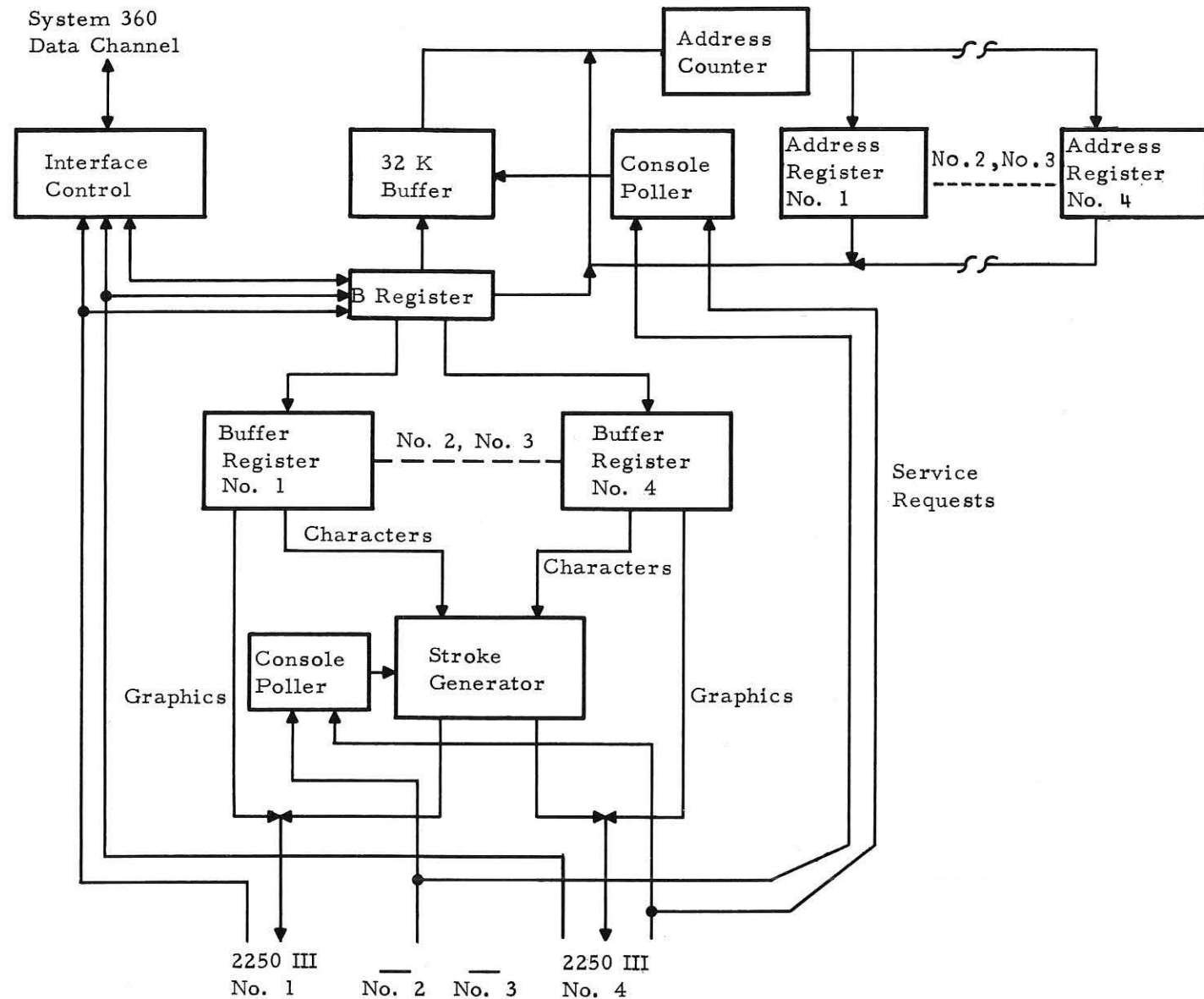
FIGURE 10: The 2840 Model II control interfaces with a System/360 computer data channel. It time-shares a buffer and stroke generator among the 2250 Model III display consoles. Two to four consoles can be attached. The control system is asynchronous in order to avoid delays for consoles not requiring buffer or stroke generator service.
