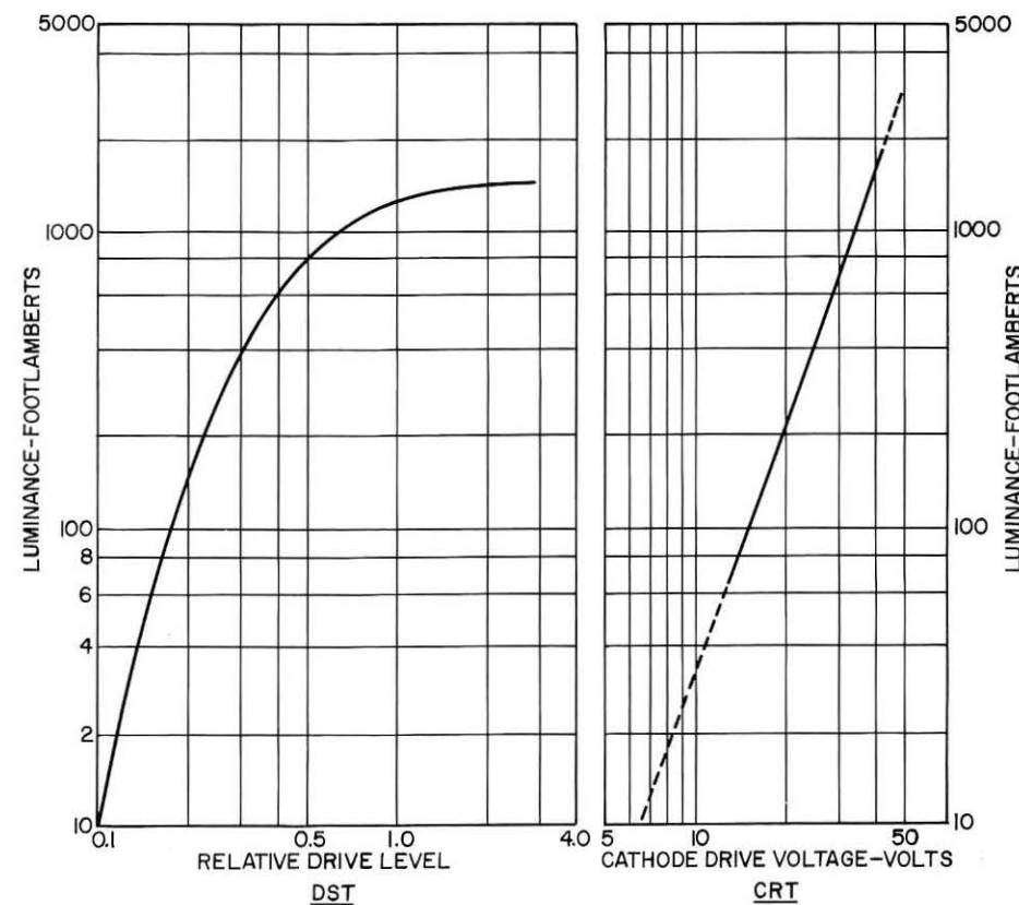
FIGURE 6: Over-all transfer characteristics.
