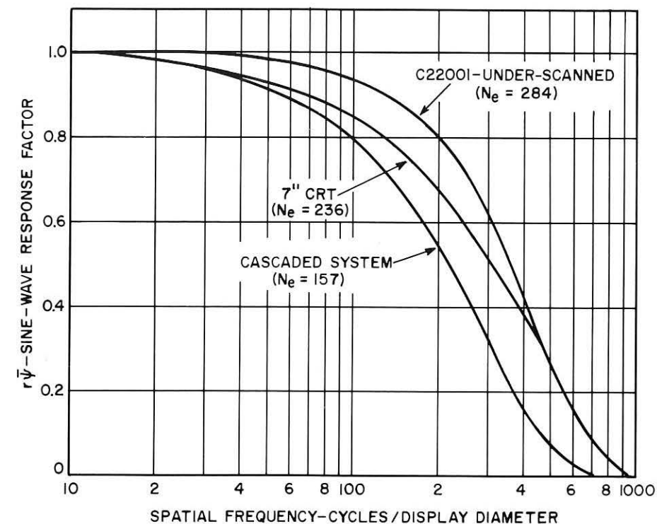
FIGURE 16: Frequency-response functions of elements of SC/CRT system, and of over-all system, in direction perpendicular to raster lines.
