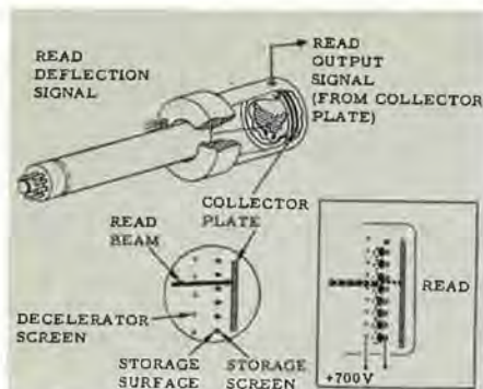
Figure 27. Reading Phase.
