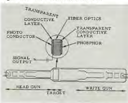
Figure 46. FOPT Scan Converter Tube.
