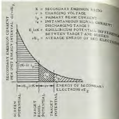
Figure 20. Writing Phase.
