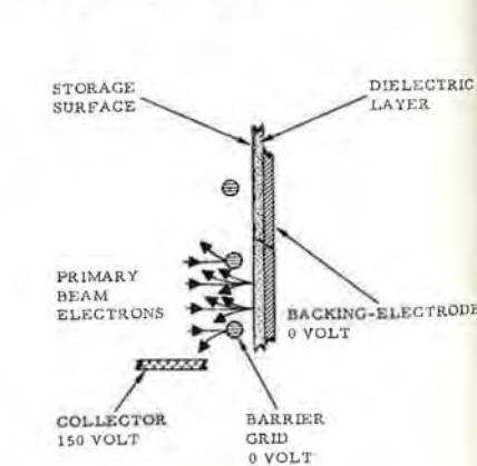
Figure 22. Erase and Prime Phase.
