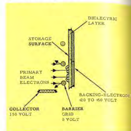
Figure 21. Reading Phase.
