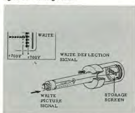
Figure 26. Writing Phase.
