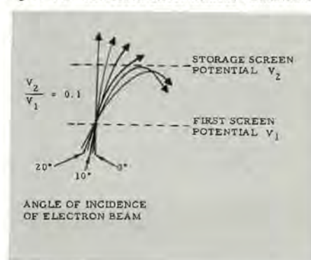
Figure 24. Refraction Effect Without Collimation.
