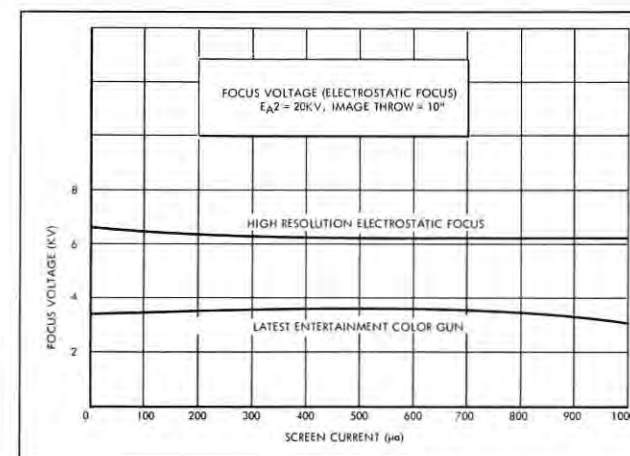
Figure 4. Curves of Focus Voltage for Entertainment Color Gun, Electrostatically Focused High Resolution Gun.
