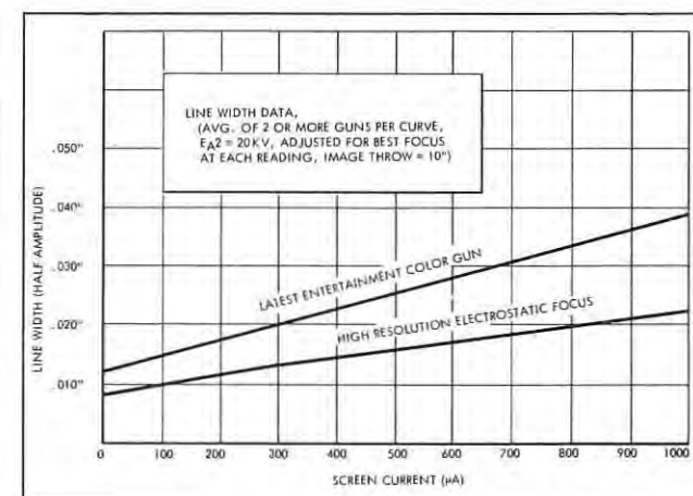
Figure 5. Curves of Line Width for Latest Entertainment Color Gun, and for Electrostatically Focused High Resolution Gun.
