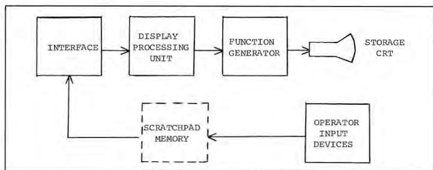
Figure 2. Storage Tube
