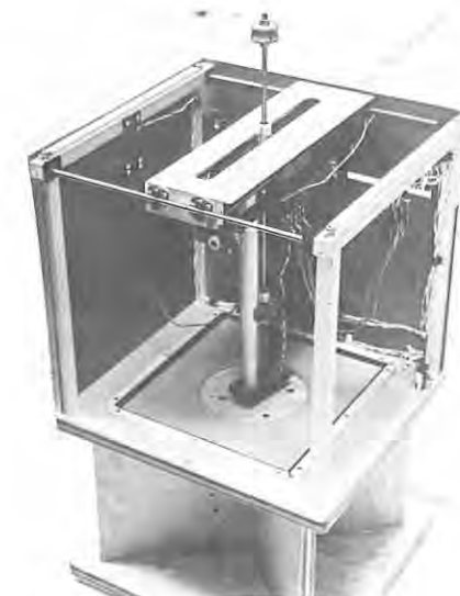
Figure 7. Photographs of a three-dimensional cartesian input device both (a) with and (b) without external covers.
