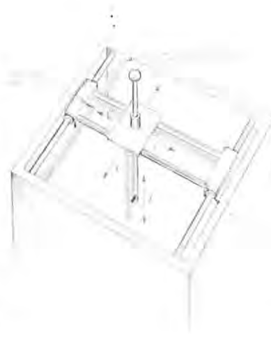
Figure 6. Sketch of a three-dimensional input device based upon a cartesian system using three mutually-perpendicular linear potentiometers.
