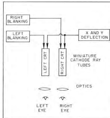
Figure 1. A stereoscopic viewing system using two miniature cathode ray tubes and blanking signals so that the image on only one of the tubes is displayed at a time.
