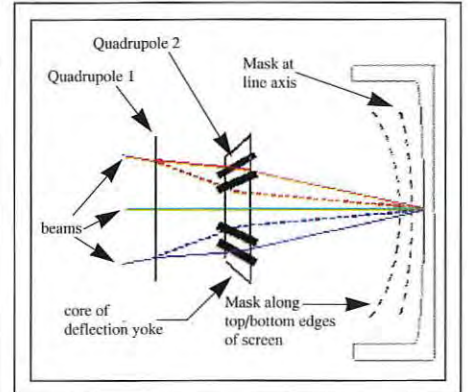
Fig. 6: Two sets of quadrupoles virtually change the gun pitch; the continuous lines represent the beams at the center of the screen, and the dashed lines represent the beams on their way to the top or bottom of the screen.
