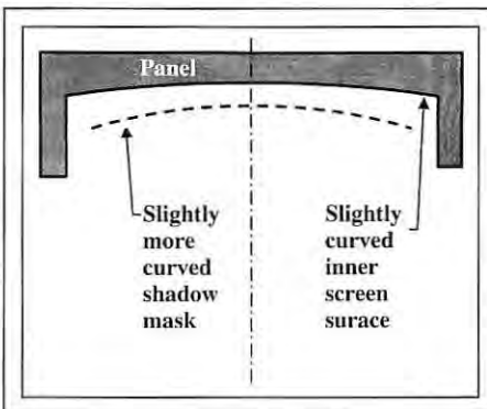
Fig. 3: This top view of the basic layout of the screen and mask of the Sony Real Flat tube shows how the mask is curved more than the screen.
