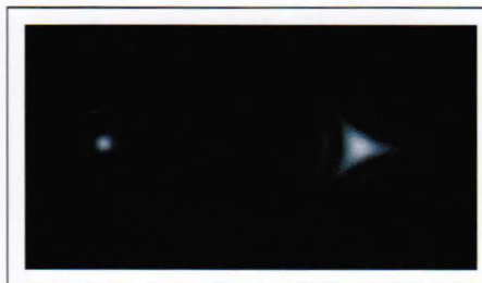
Fig. 5: The effect of improved mirror design is apparent in these two pixel spot images – normalized for size but not for intensity – for a scanned spot at \sim\lambda/4 p-p mechanical mirror deformation (left image) and a scanned spot at \sim 2\lambda p-p mechanical mirror deformation (right image).
