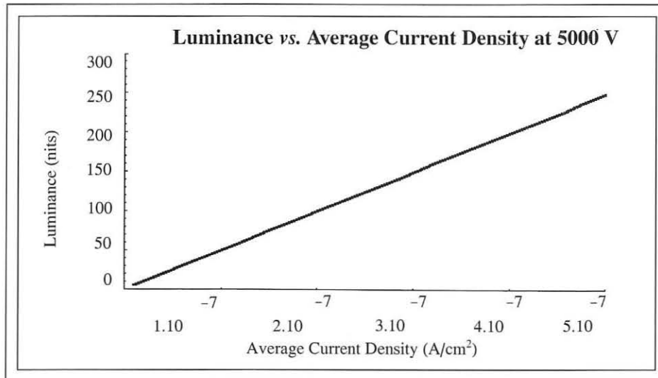
Fig. 5: Calculated plot of the luminance (nits) vs. average current density (A/cm²) for a green ZnCdS:Cu,Al phosphor operating at 5000 V with a 2-μsec pulse width. The duty factor is 1/1440 and the average current can be found by multiplying by 1440.
