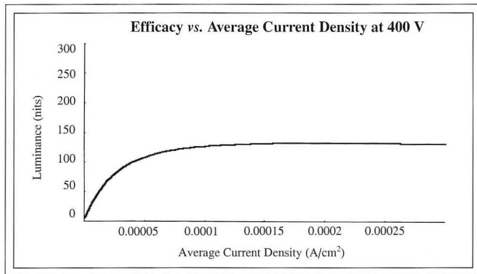
Fig. 4: Calculated plot of the luminance (nits) vs. average current density ( A/cm^2 ) for a green ZnCdS:Cu,Al phosphor operating at 400 V with a 2- \mu sec pulse width. The duty factor is 1/1440 and the peak current can be found by multiplying by 1440.
