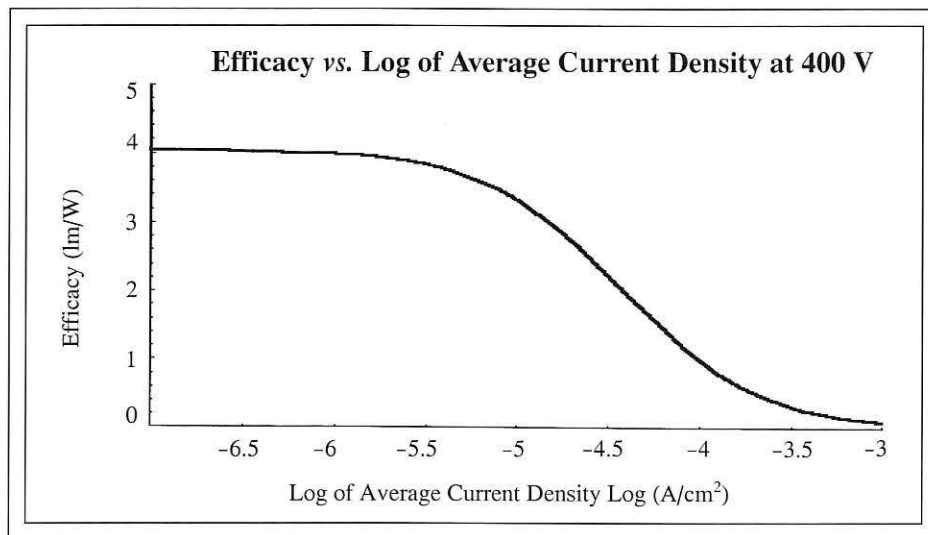
Fig 2: Calculated plot of the efficacy (lm/W) vs. log of the average current density ( A/cm^2 ) for a green ZnCdS:Cu,Al phosphor operating at 400 V with a 2- \mu sec pulse width. The duty factor is 1/1440 and the peak current can be found by multiplying by 1440.
