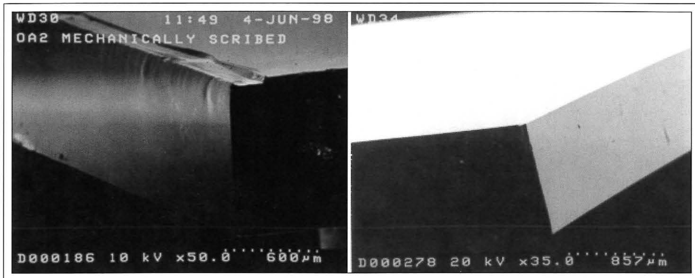
Fig. 1: A typical laser-cut edge is cleaner and more strain-free than a mechanically cut edge.
