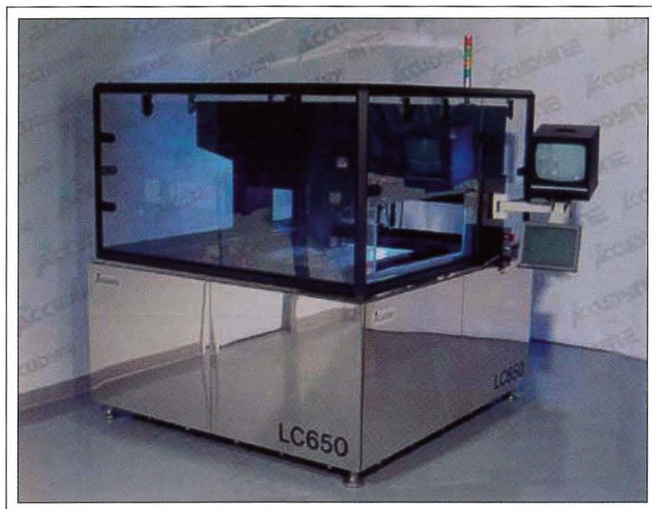
Fig. 2: The LC-650 beta laser cutting tool was developed under a contract with the United States Display Consortium.
