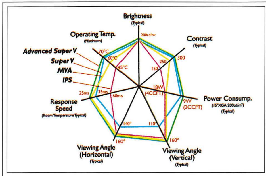
Fig. 3: Mitsuki Hirata, Noriko Watanabe, Motohiro Yamahara, and Shigeaki Mizushima used this process to model LCD and compensating-film performance.
