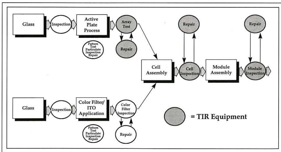
Fig. 1: This general overview of LCD fabrication shows where inspection, test, and repair fit into the manufacturing process.
