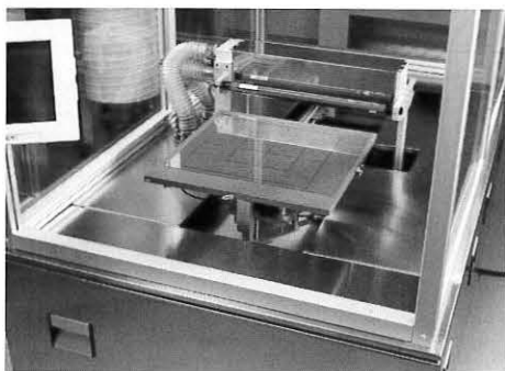
Stand Alone Non-Contact Dry Cleaning Module: Eliminates 95% of particles greater than 1 micron. High frequency pressure waves from an ultrasonic head cause particles to vibrate which are then removed by an exhaust airflow.
